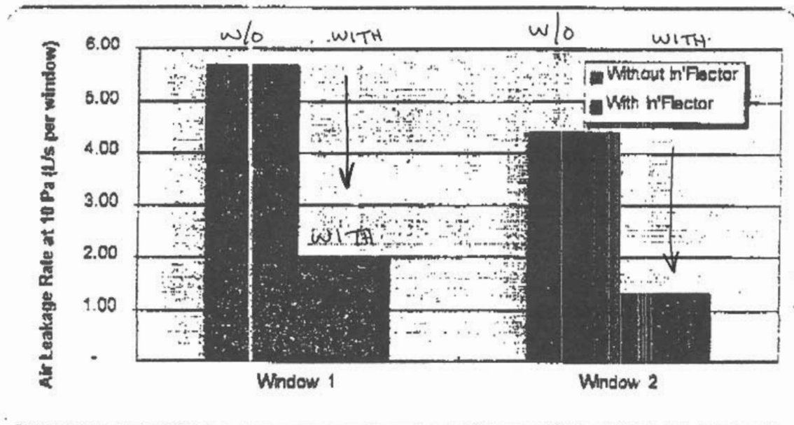
Figure 1: Improvements in the air leakage behavior of windows with the use of In'Flector panels at the normal operating conditions in the building.
